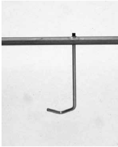
Figure 15 – Two good features of a hook: sharp bottom and TIG weld on far side of drilled mount hole.
