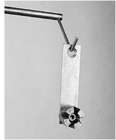
Figure 17 – Magnet tab for mounting steel parts lacking holes onto conventional rack hooks.
