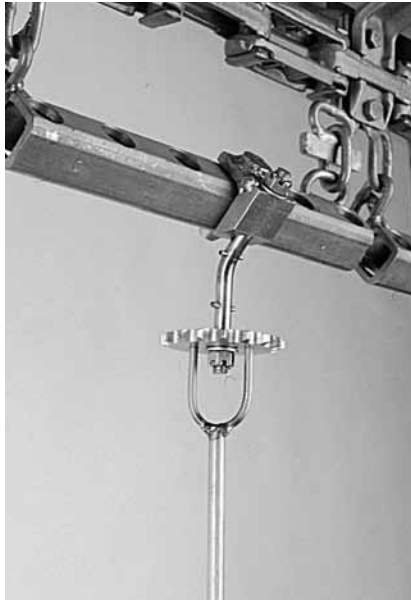
Figure 8 – Non-recoil automatic rotator. Contact point with drive gear rack is on extended centerline of Angle Pivot™ bearing.
