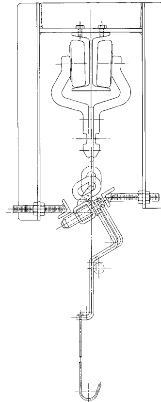
Figure 11 – Hold-Down tracks are sometimes used with paired workholder hooks (see Figure 6).
