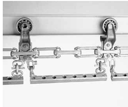
Figure 1 – Continuous load bar Angle Pivot™ installation on X-458 short-drop conveyor. Trolley spacing = 16".
