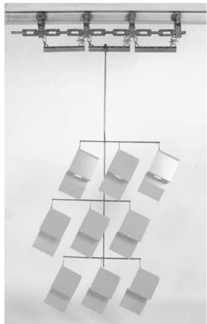
Figure 14 – Asymmetric rack with diagonal columns of parts. Saves on vertical envelope space.
