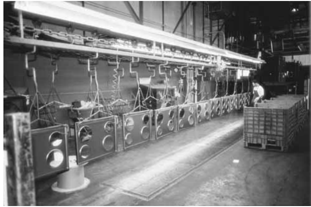
Figure 1 – Present main top loading area after installation of Angle Pivoting hanging system.
