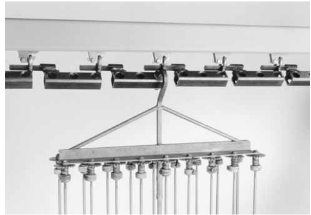
Figure 15 – Power rotators for small round parts, built into the proper configuration for angle pivot use.
