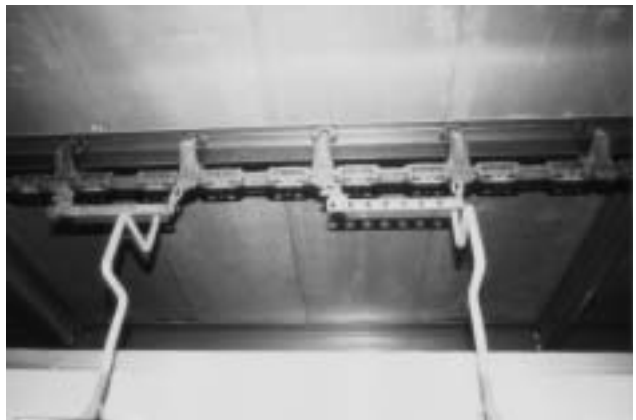
Figure 3. A close up view of the Angle Pivoting system.
