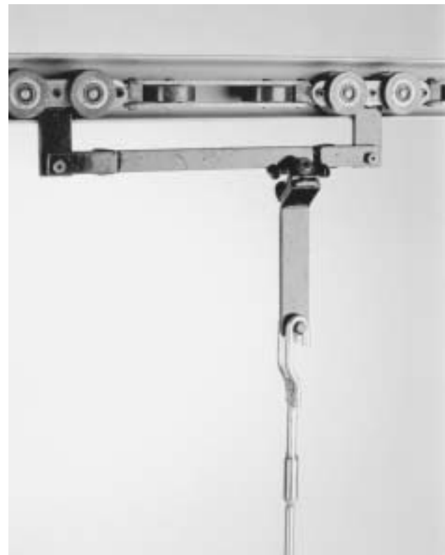
Figure 5. Compound: A load bar between two hang points, with a single payload mount bearing on or off the centerline.
